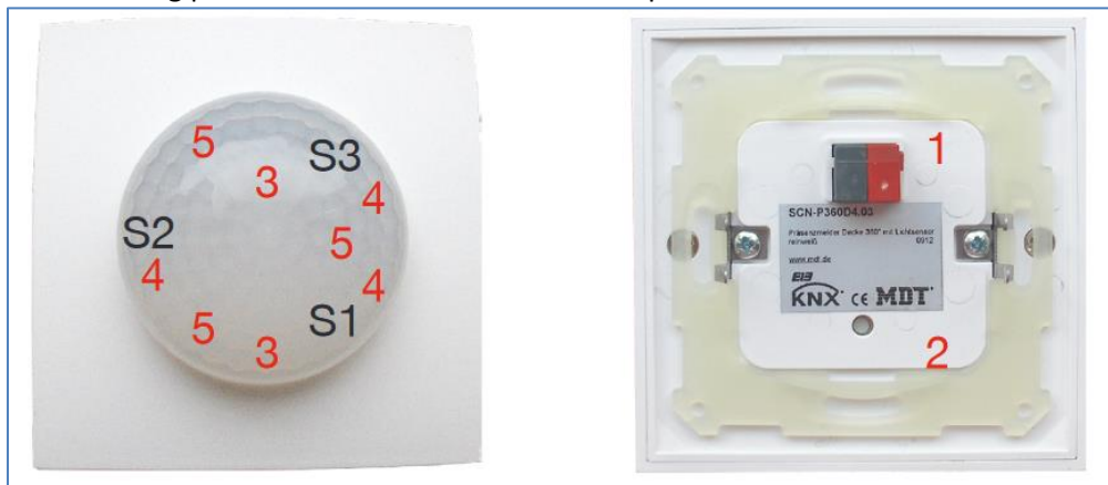
Figure 3: Structure and location of the sensors/LEDs – SCN-P/G360x3.03
