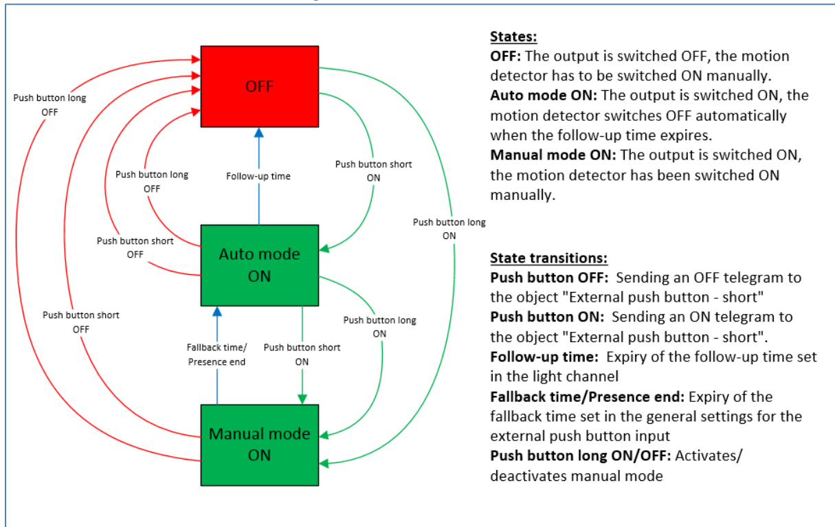
Figure 22: Process diagram – Half automatic without orientation light
