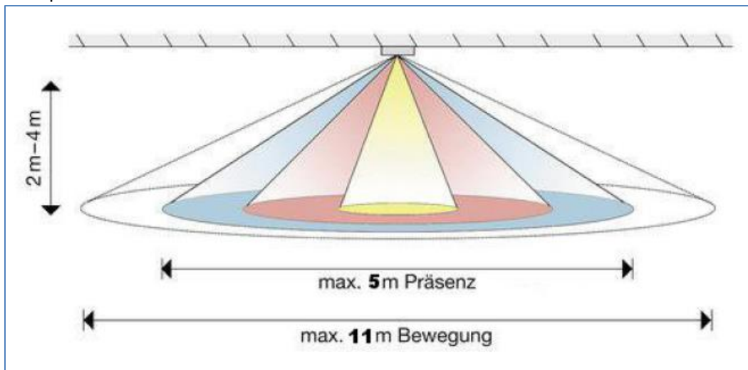
Figure 6: Detection area SCN-P360x3.03
