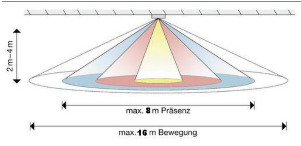
Figure 5: Detection area SCN-P360x4.03
